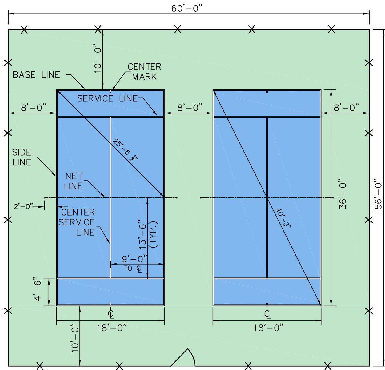
TWO COURT LAYOUT (NEW CONSTRUCTION)
