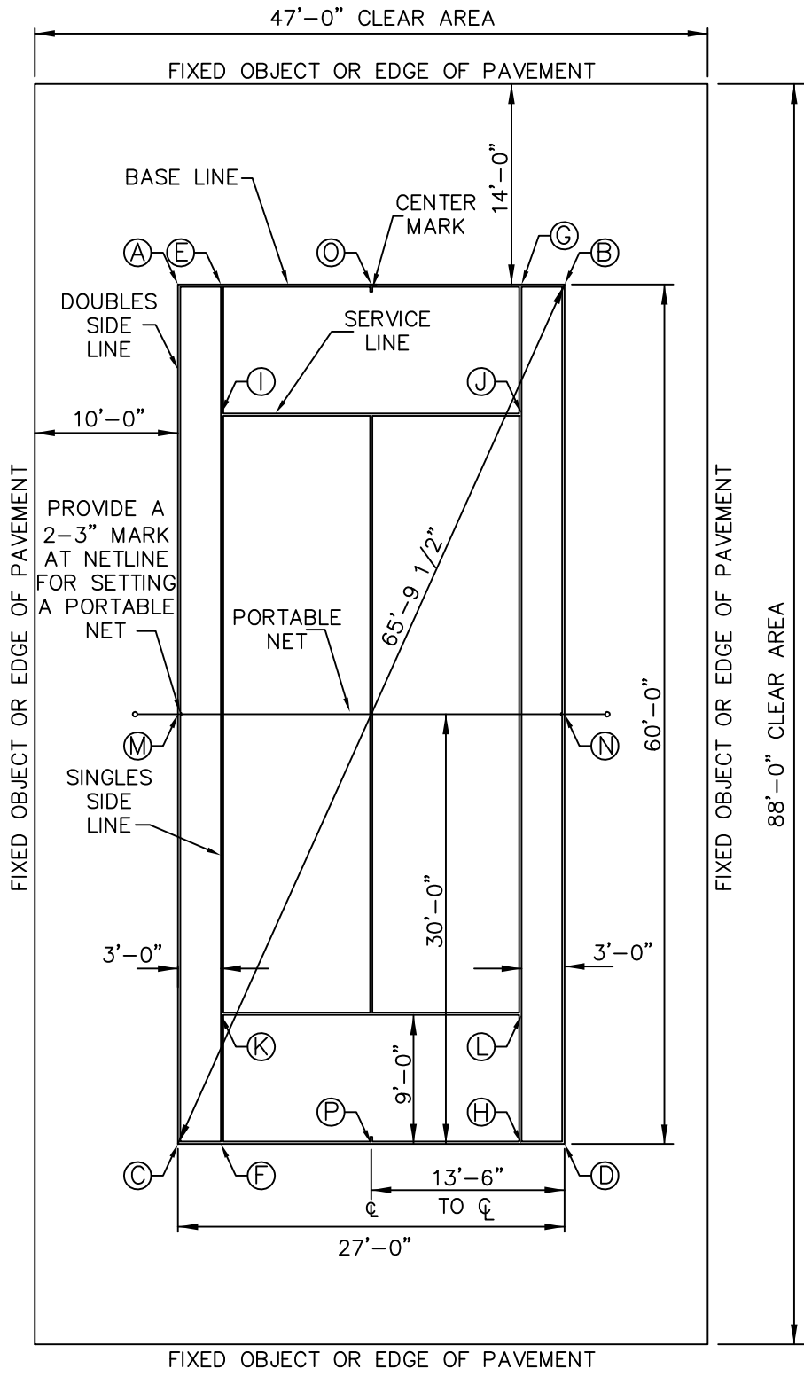
SINGLE COURT LINE LAYOUT NOT TO SCALE
