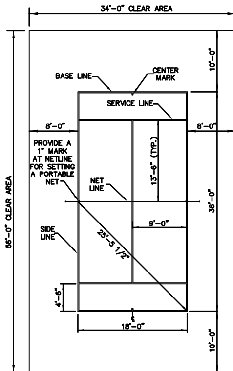
SINGLE COURT LAYOUT
