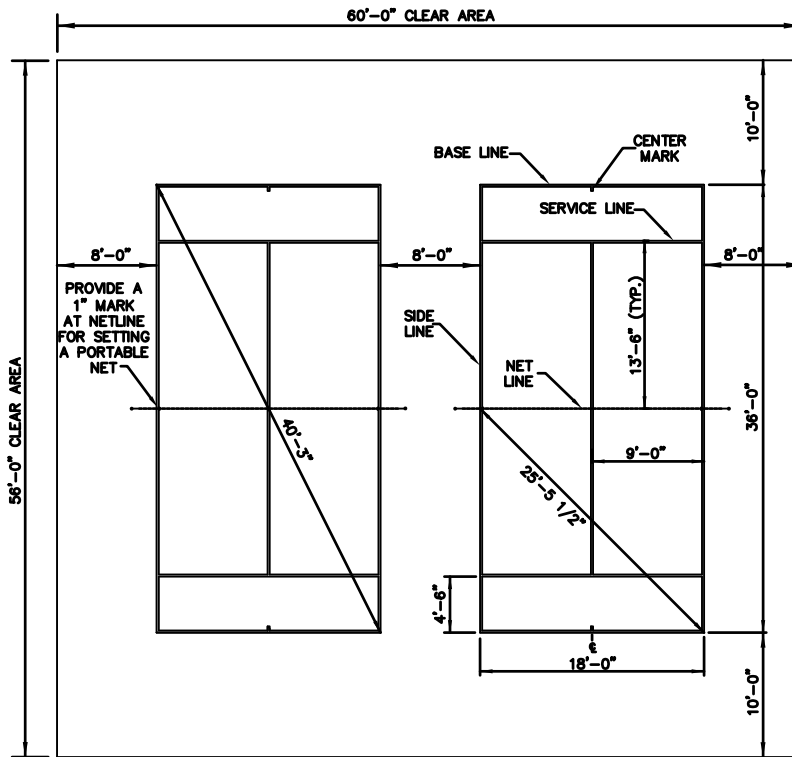
TWO COURT LAYOUT
